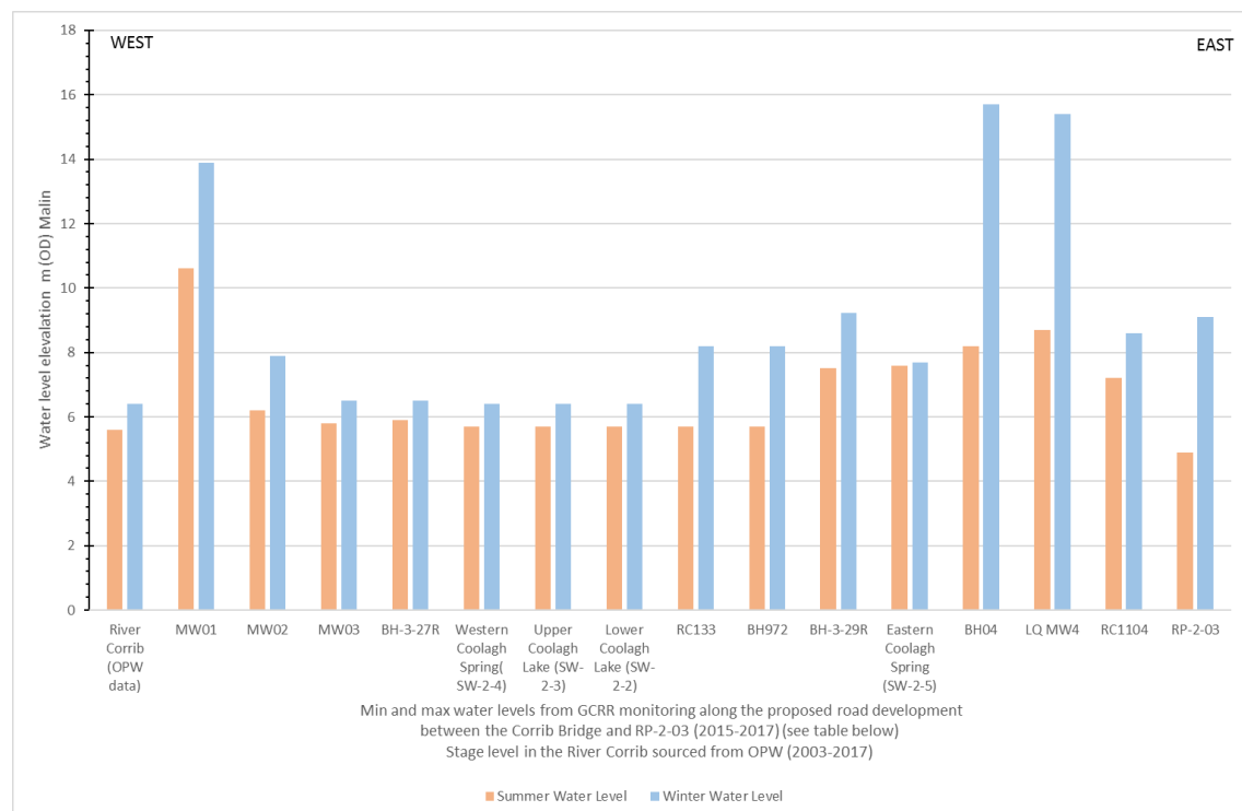
Plate 4: Groundwater levels in the vicinity of S19B
