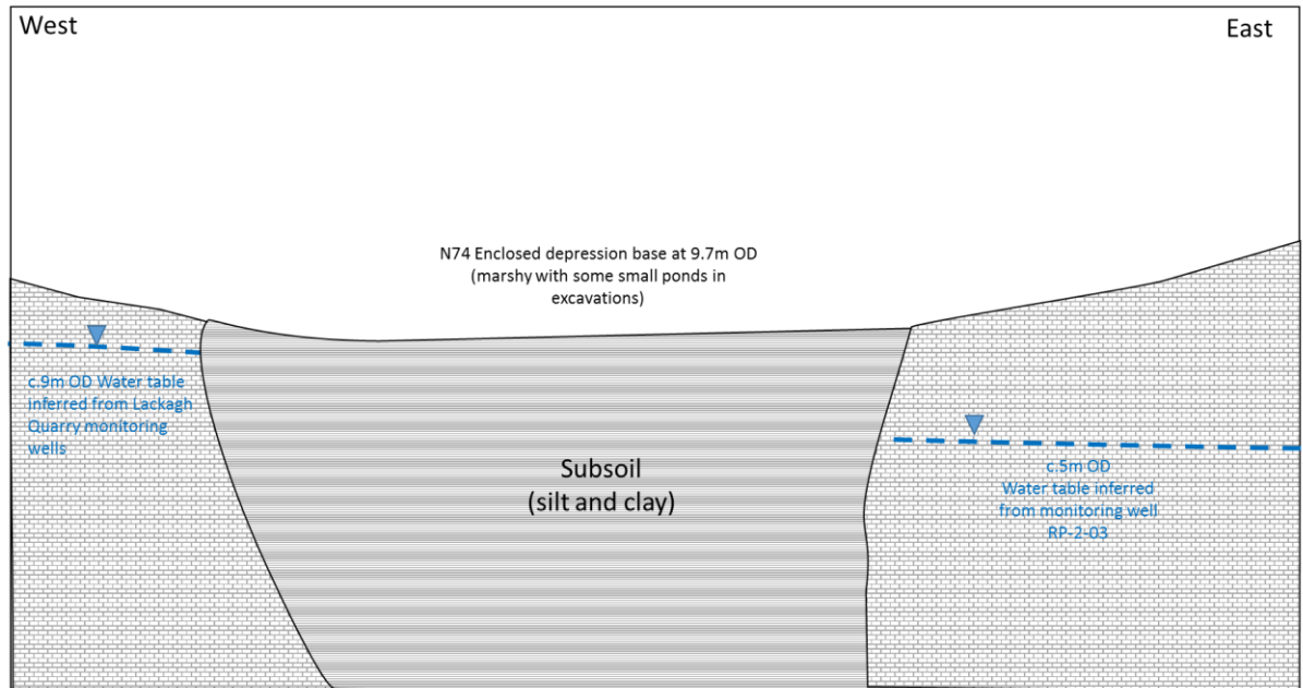
Plate 9: Conceptual hydrogeology at Lake at Ballinfoyle during high (winter) groundwater levels
