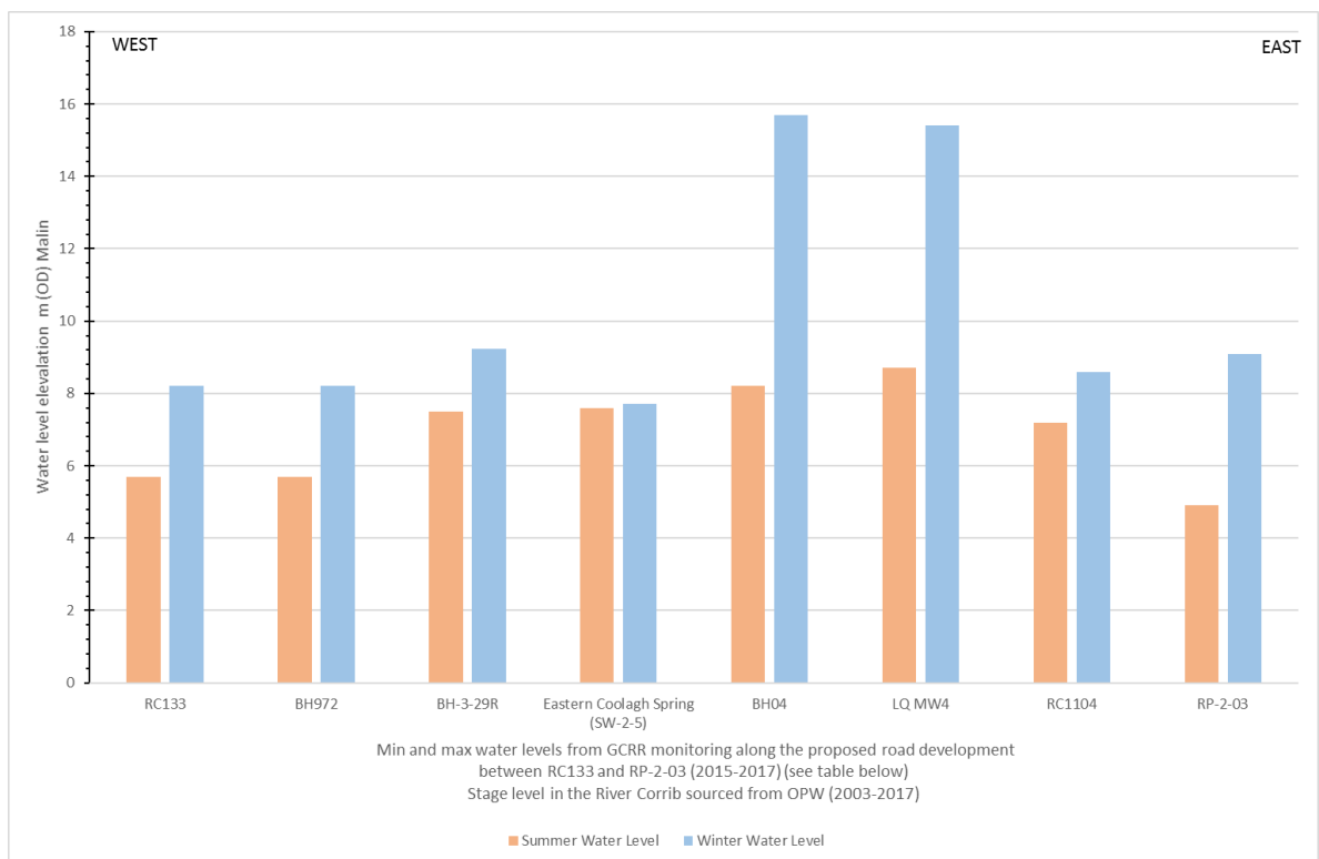
Plate 7: Groundwater levels in the vicinity of S20
