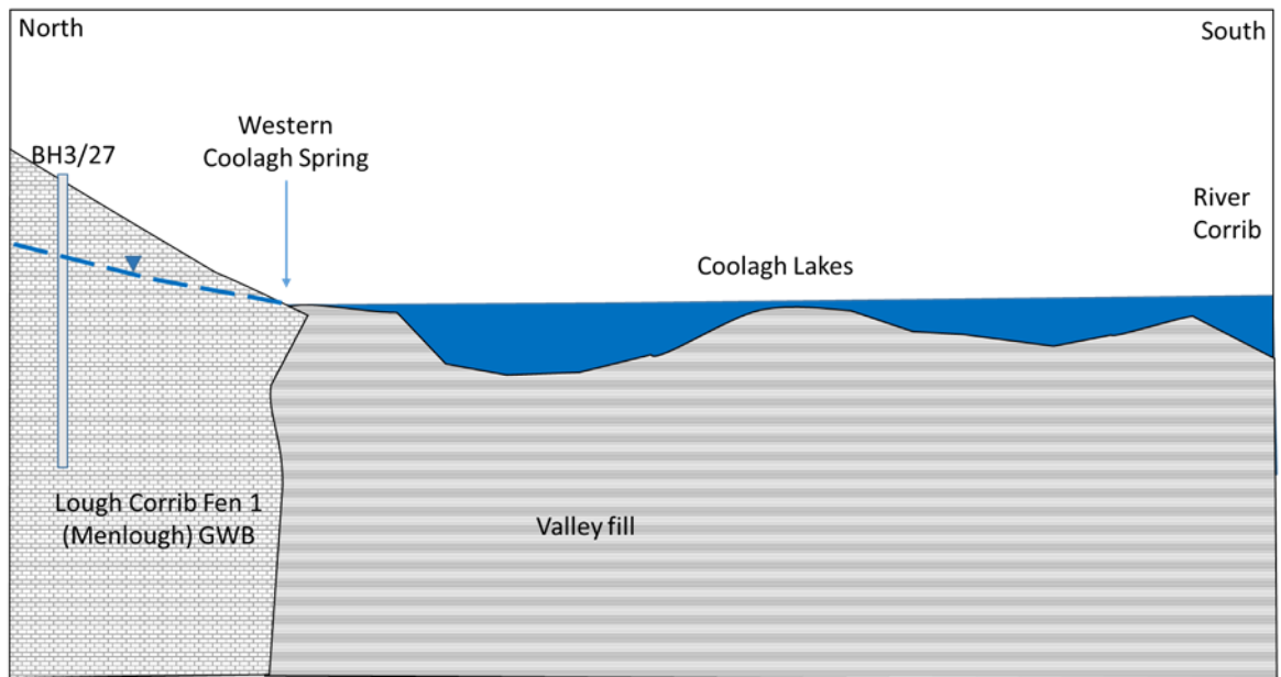
Plate 15: Schematic north south cross-section through Coolagh Lakes (groundwater high)
