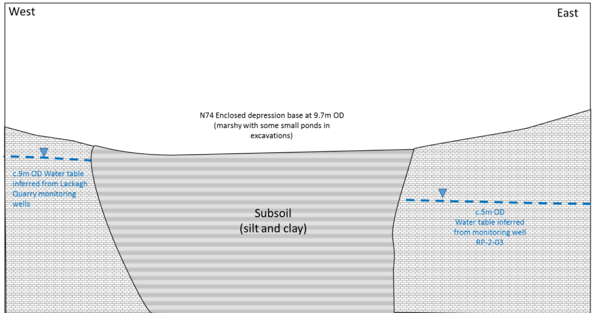
Plate 10: Conceptual hydrogeology of the lake at Ballinfoyle during low (summer) groundwater levels
